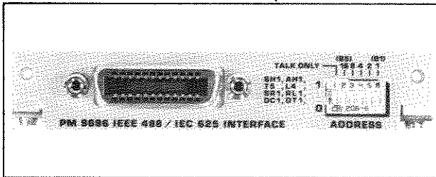
Fig. 5.1 Bus Interface panel.
