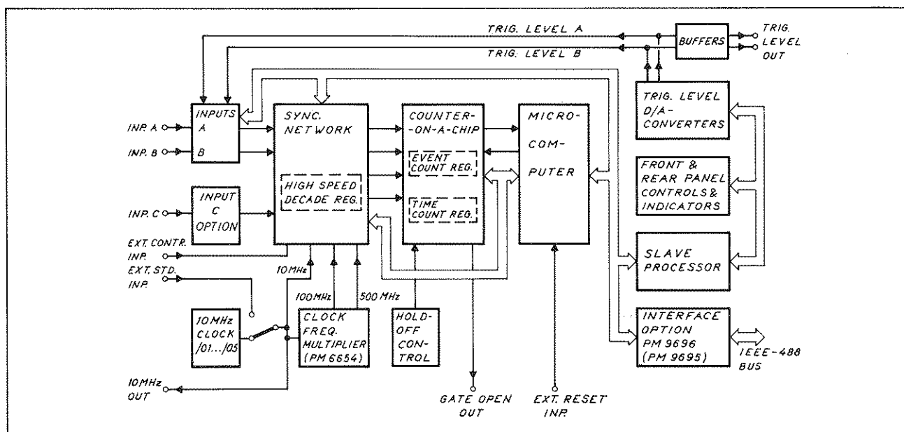
Fig. 7.1 Block diagram PM 6652/54
