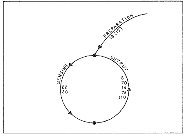
Fig. 5.8 Measuring cycle: TOTALIZE A.
